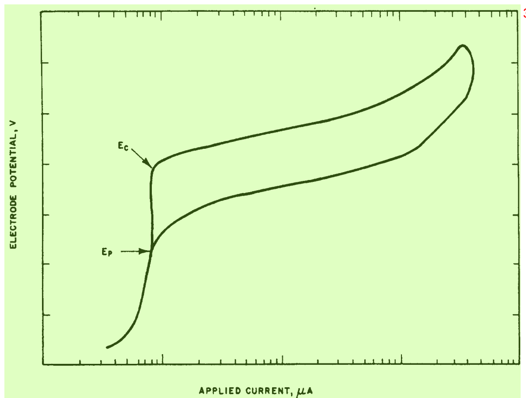
FIGURE 3 — Schematic representation of a cyclic potentiodynamic anodic polarization curve for SSs in halide media.
